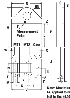
L002a TO-218 x Weight = 5.2 g
