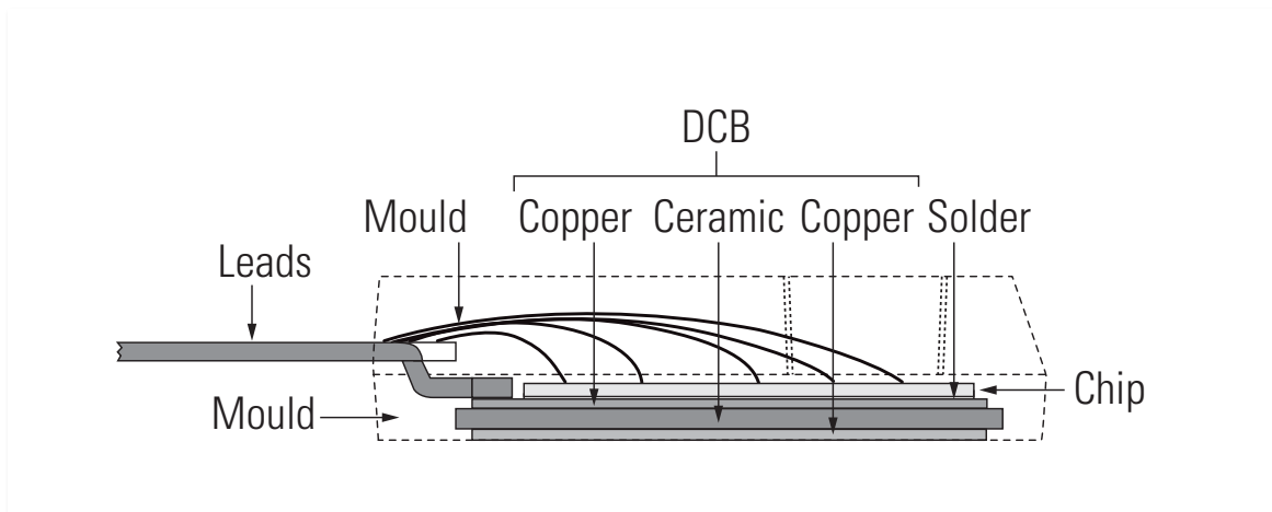
Package Cross-Section
