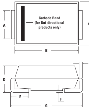
L003b DO-214AB Weight = 0.2 g
